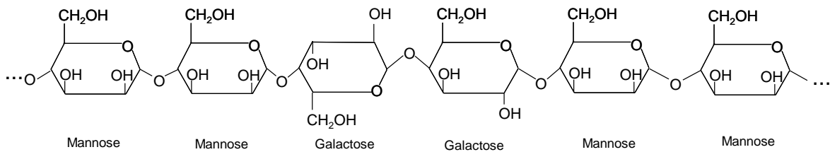
Mannose
